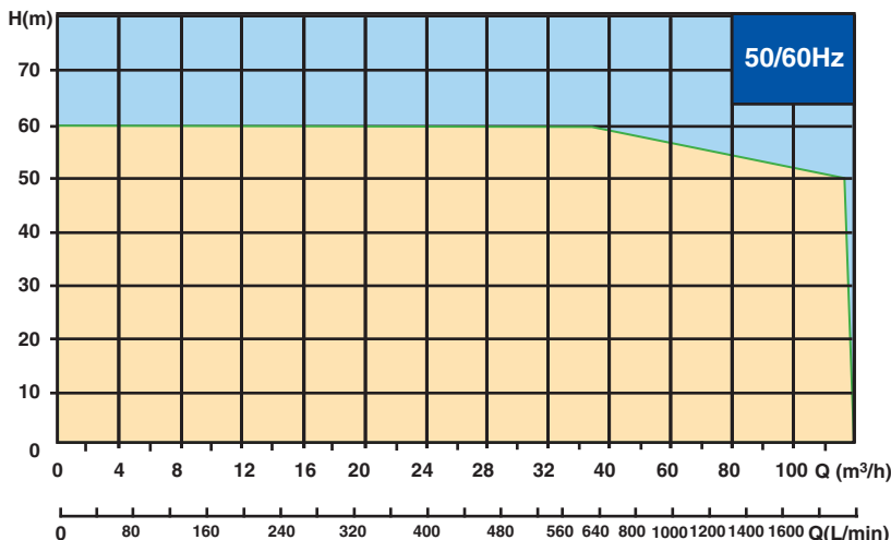
Performance Curves - CGW 4200/500/6600
